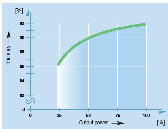
Fig. 4: Efficiency as function of output power
